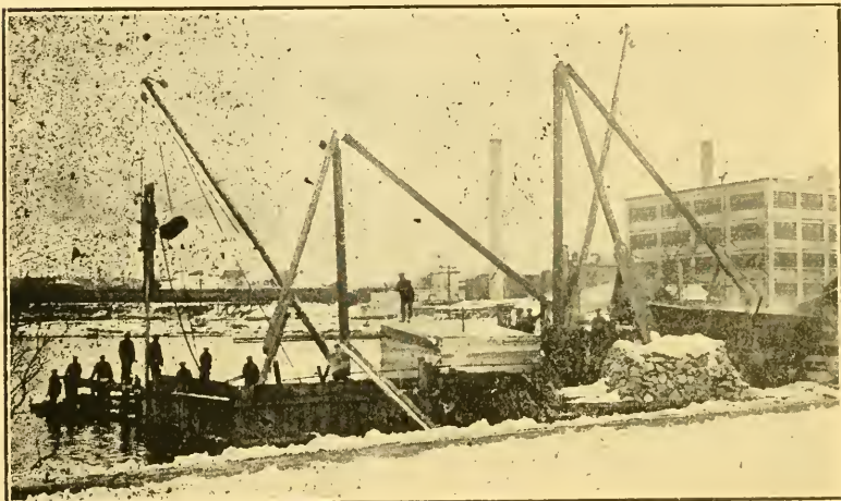
Caissons and foundations for Turners Falls Power & Electric Co. at Silver Lake, Pittsfield, Mass.
